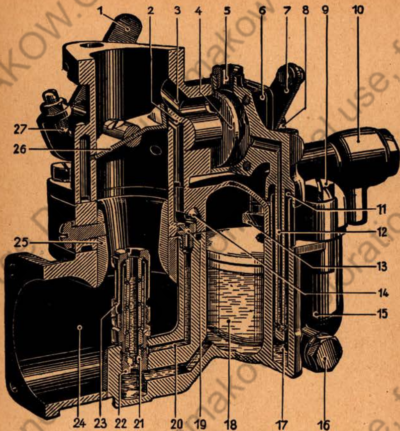
Steigstromvergaser (Solex 35 BFLV)
